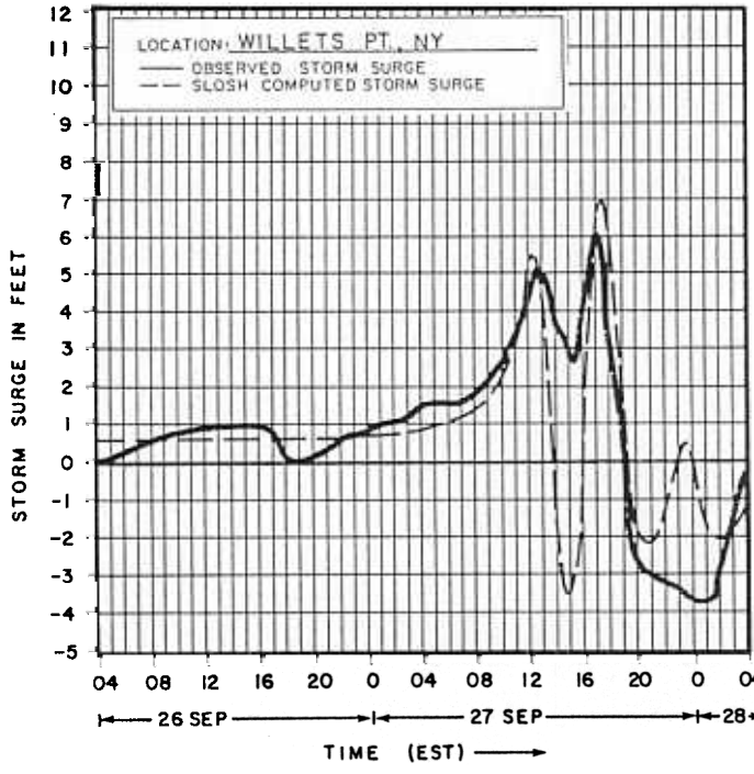
Figure 8a. Comparison of observed versus SLOSH model computed storm surge hydrographs for four locations in Figure 5.
